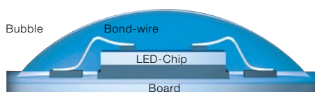
Chip-on-board LED: light distribution is defined by the shape of the bubble.
