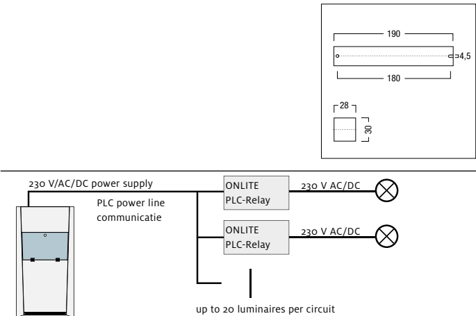
ONLITE central PLC DALI Relais
