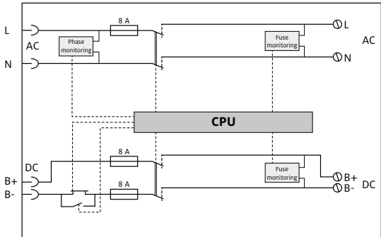
SCM Switch connection module
